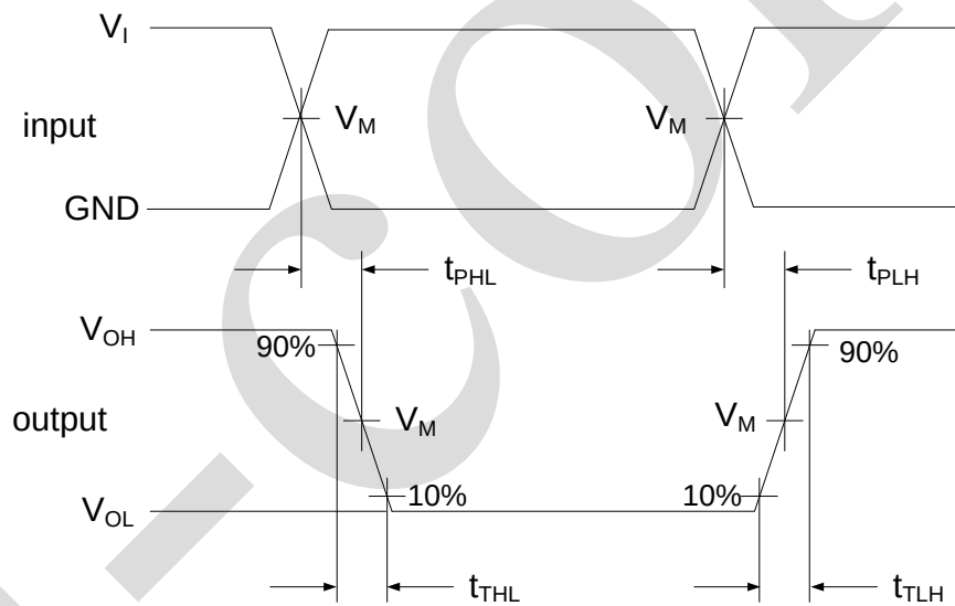
Figure 5. The data input (A) to output (Y) propagation delays
