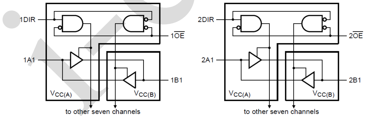
Figure 2. Logic diagram
