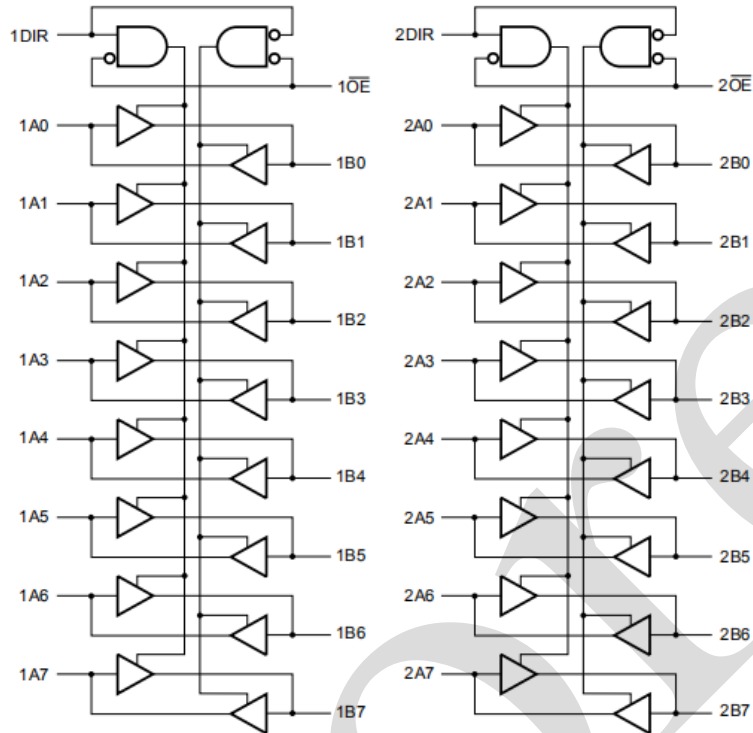
Figure 1. Logic symbol
